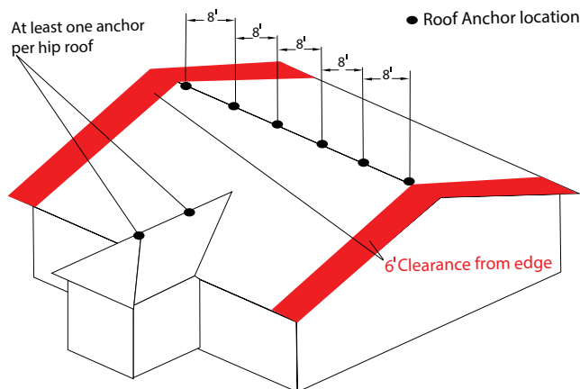
ANCHOR ROOF LOCATIONS (FIG.1)
